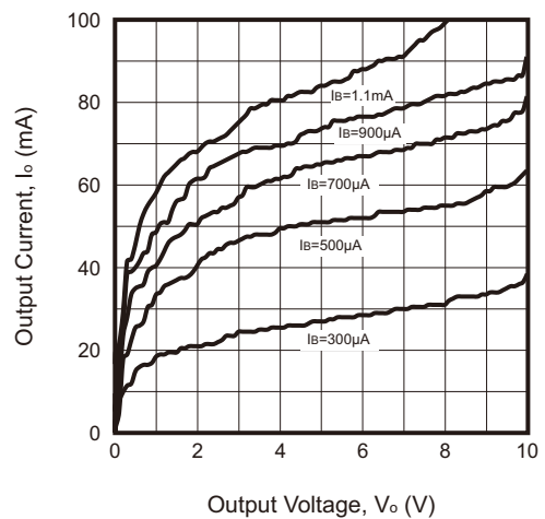
Fig.5 - Output Current vs. Output Voltage
